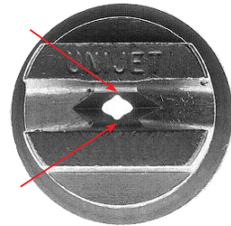
Figure 7.1.2 b Worn out nozzle
