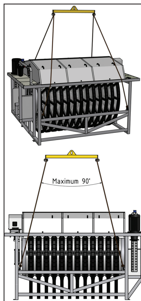
Figure 3.3 Lifting points for filters without tank (type 2/3)
