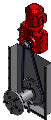
S77DRE90M4 M4A on mirrored filters Art. no. 1014653
