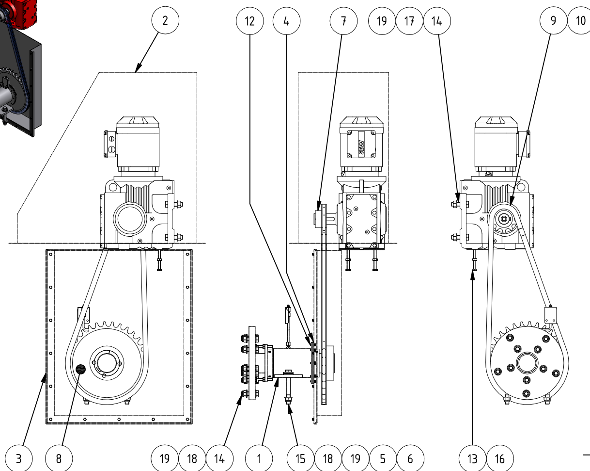
S77DRE90M4 M4A on mirrored filters Art. no. 1014653
